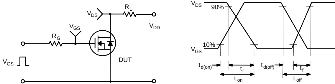
Figure 14. Resistive Switching Test Circuit &amp; Waveforms
