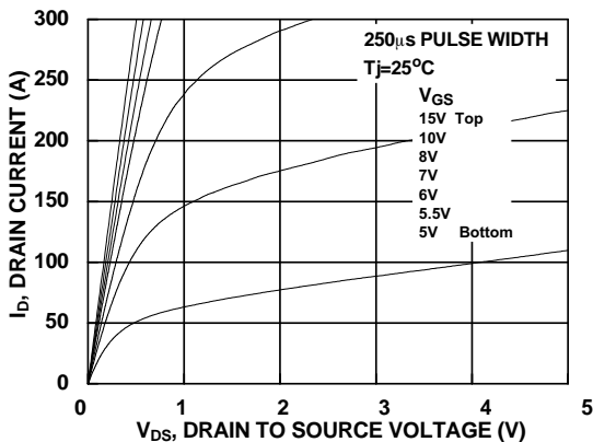
Figure 9. Saturation Characteristics
