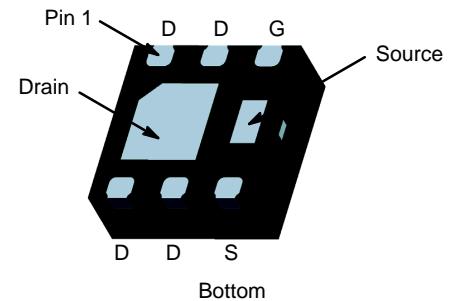
WDFN6 2x2, 0.65P (MicroFET 2x2) CASE 511CZ
