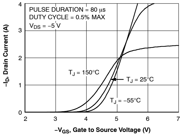
Figure 18. Transfer Characteristics
