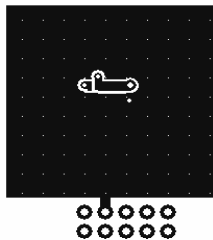
a. 50\text{ }^\circ\text{C}/\text{W} when mounted on a 1 in 2 pad of 2 oz copper.
