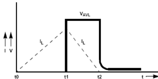
Figure 4. Avalanche Current and Voltage Definitions
