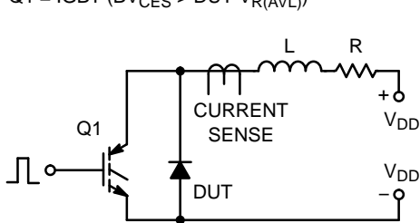
Figure 10. Unclamped Inductive Switching Test Circuit & Waveform
