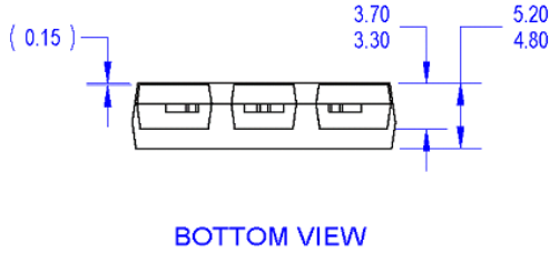
Figure 23. TO264, Molded, 3-Lead, Jeduc Variation AA
