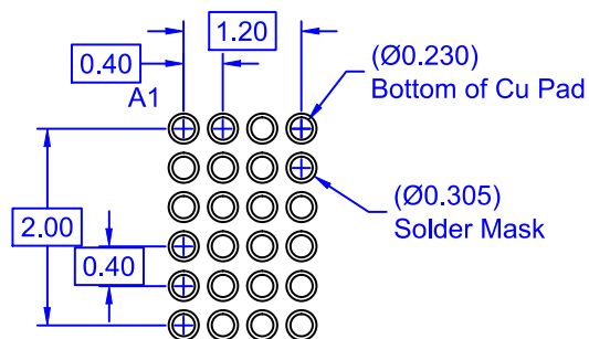
RECOMMENDED LAND PATTERN (NSMD PAD TYPE)
