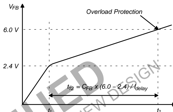
Figure 20. Overload Protection
