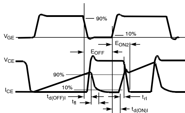
Figure 20. SWITCHING TEST WAVEFORMS
