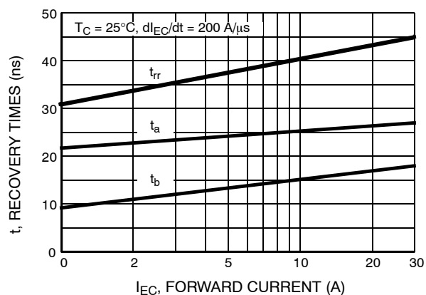
Figure 18. RECOVERY TIMES vs. FORWARD CURRENT
