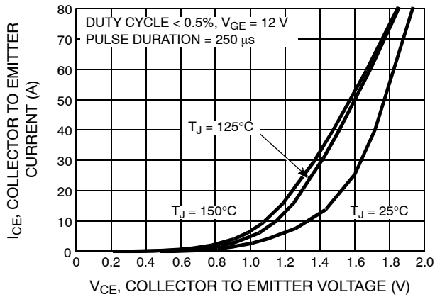
Figure 5. COLLECTOR TO EMITTER ON-STATE VOLTAGE
