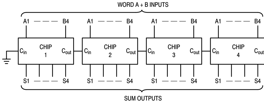
Figure 5. Logic Diagram
