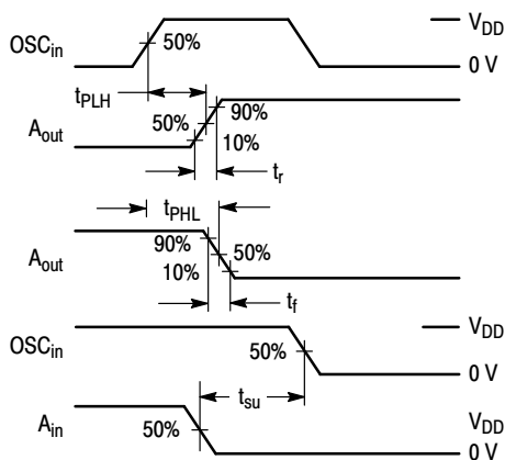
Figure 1. Switching Waveforms
