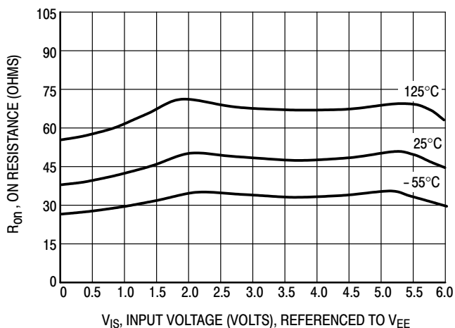
Figure 8. Typical On Resistance, V_{CC} - V_{EE} = 6.0 \text{ V}
