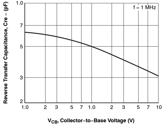
Figure 4. C_{re} - V_{CB}
