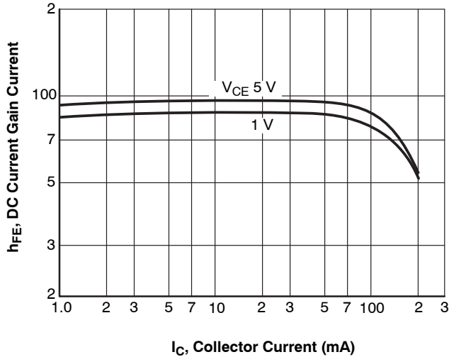
Figure 3. h_{FE} - I_C
