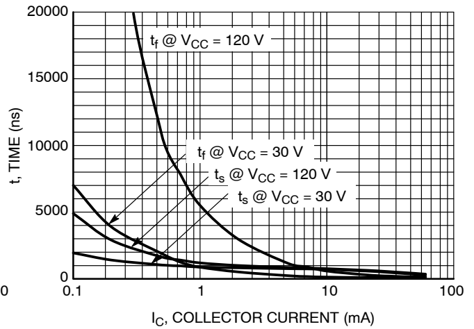
Figure 14. Turn-Off Time
