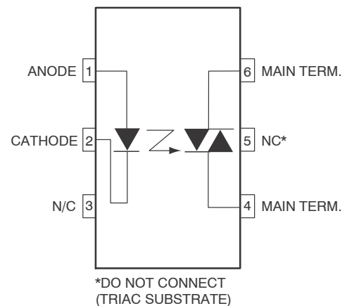
Figure 1. Schematic
