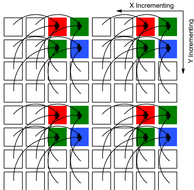
Figure 20. Pixel Readout (Column and Row Binning)
