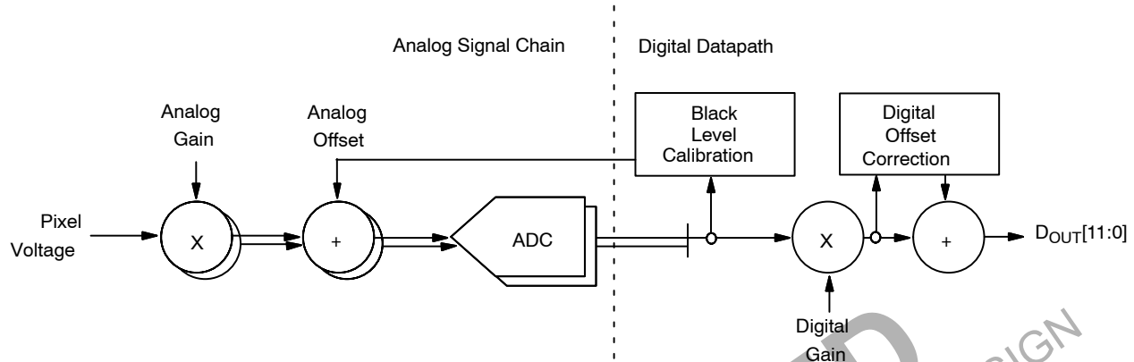
Figure 25. Signal path
