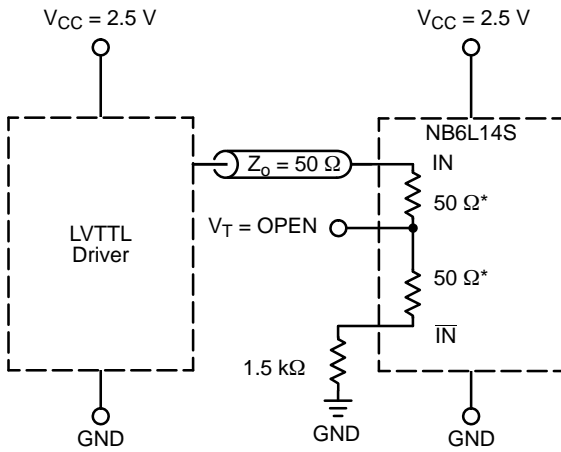
Figure 16. LVTTL Interface
