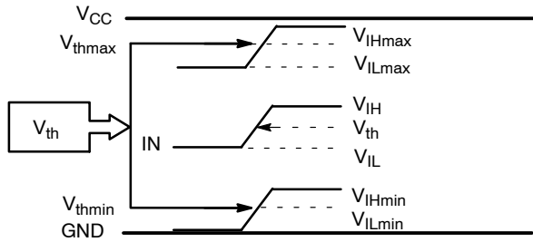
Figure 9. V_{th} Diagram
