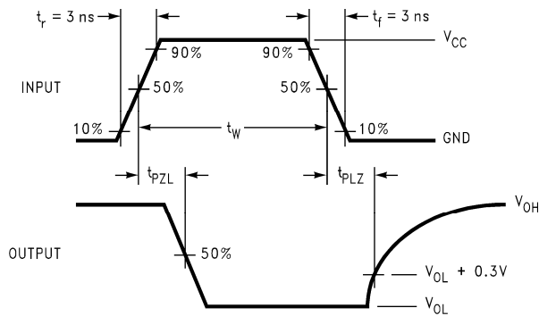
Figure 5. AC Waveforms
