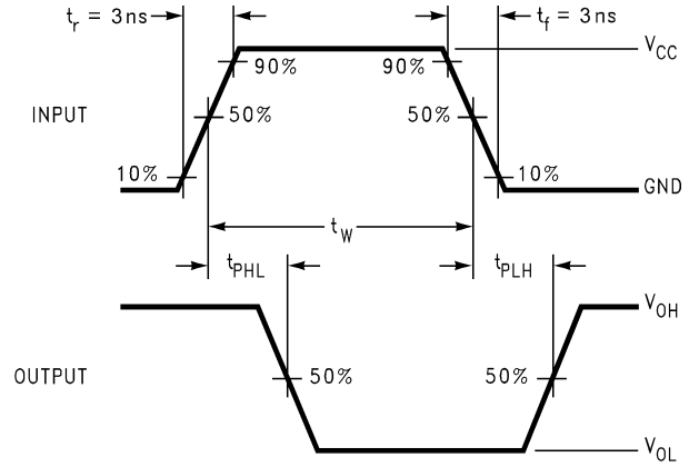
Figure 7. AC Waveforms
