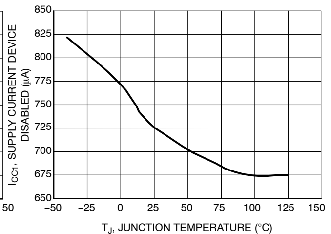
Figure 31. Supply Current Device Disabled (Overload) vs. Junction Temperature
