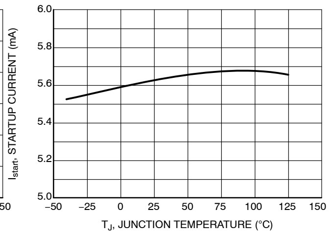
Figure 29. Startup Current vs. Junction Temperature
