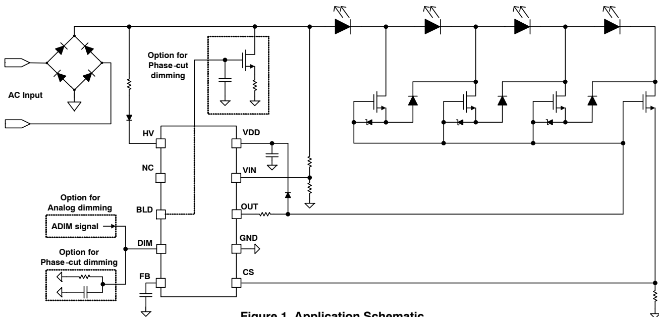
Figure 1. Application Schematic
