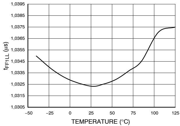
Figure 41. t_{FF1LL} vs. Temperature
