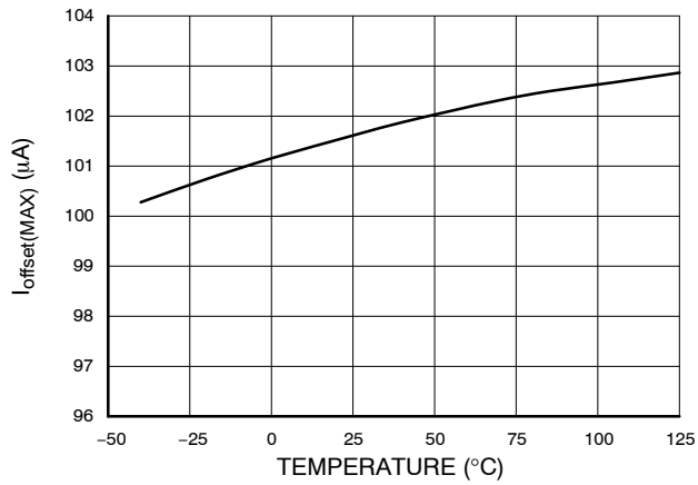
Figure 39. I_{offset(MAX)} vs. Temperature
