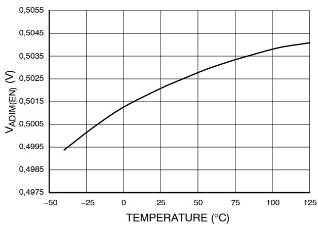
Figure 43. V_{ADIM(EN)} vs. Temperature
