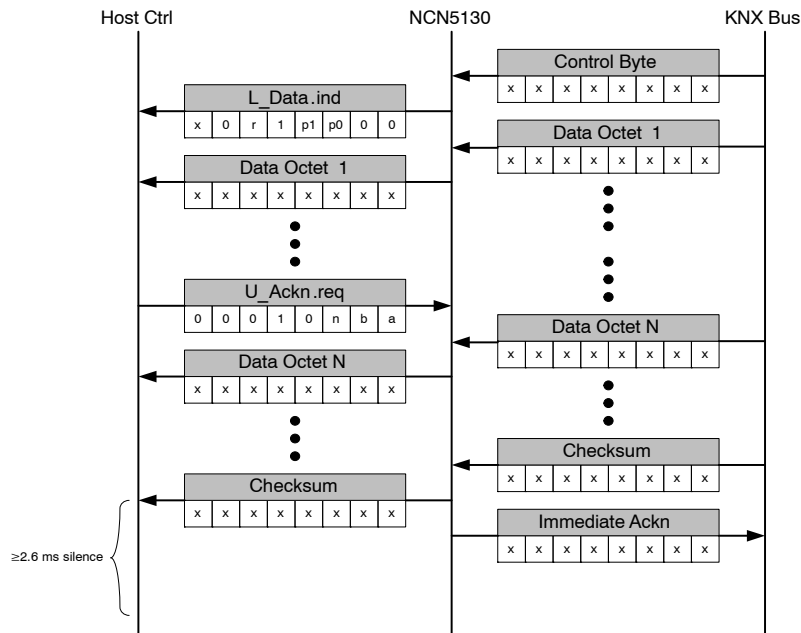
图 51. Receive Frame, 9-bit UART Mode, Frame End with Silence, No CRC-CCITT
