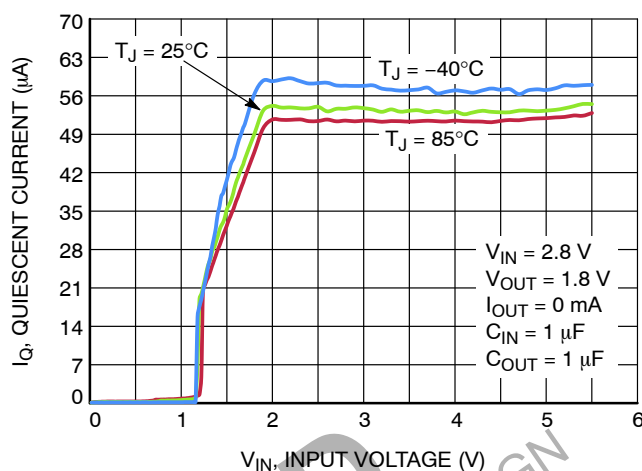
Figure 10. Quiescent Current vs. Input Voltage V_{OUT} = 1.8 \text{ V}
