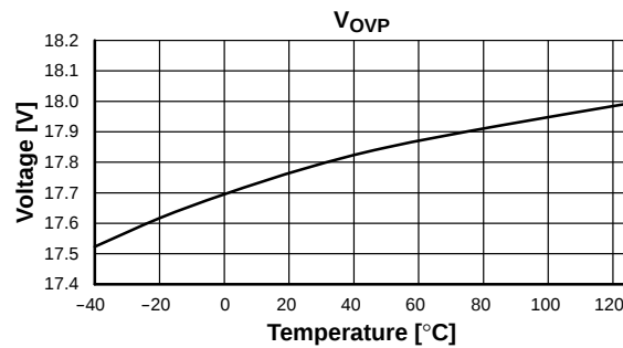
Figure 27. V OVP vs. Temperature
