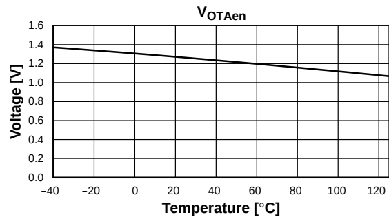
Figure 29. V OTAen vs. Temperature
