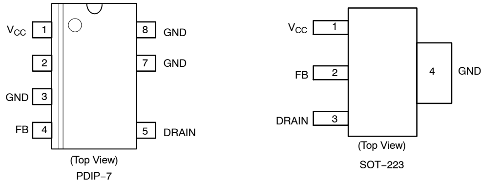
Figure 1. Pin Connections
