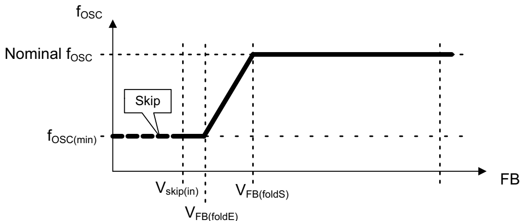
Figure 46. Frequency Foldback when the FB Voltage Decreases
