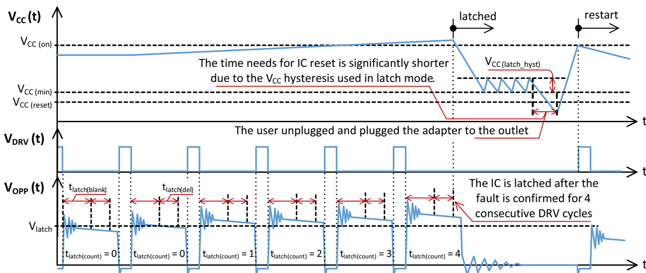
Figure 59. Latching off the controller and resuming operation.
