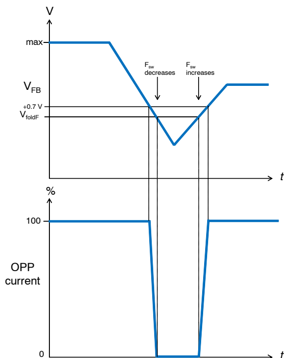
Figure 38. The OPP current is applied when the feedback voltage exceeds the foldback point. It is 0 below it
