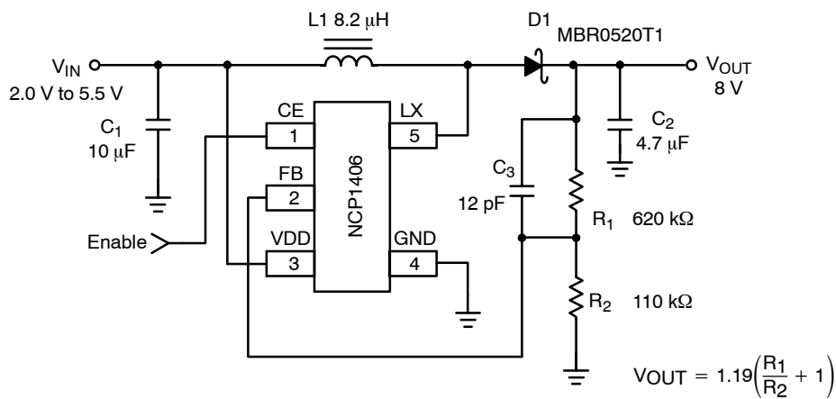
Figure 5. Typical 8 V Step-Up Application Circuit
