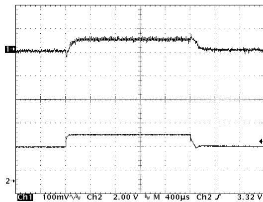
Figure 24. Line Transient Response ( V_{OUT} = 15\text{ V} )
