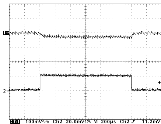
Figure 23. Load Transient Response ( V_{OUT} = 15\text{ V} )
