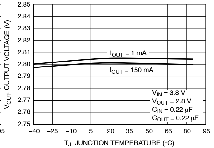
Figure 4. Output Voltage vs. Temperature V_{OUT} = 2.8 \text{ V}
