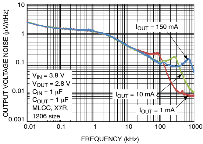
Figure 30. Output Voltage Noise Spectral Density for V_{OUT} = 2.8 \text{ V} , C_{OUT} = 1 \mu\text{F}
