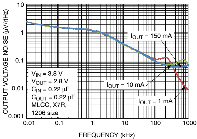
Figure 29. Output Voltage Noise Spectral Density for V_{\text{OUT}} = 2.8\text{ V} , C_{\text{OUT}} = 220\text{ nF}
