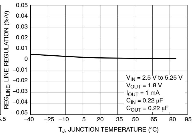
Figure 8. Line Regulation vs. Temperature V_{OUT} = 1.8 \text{ V}
