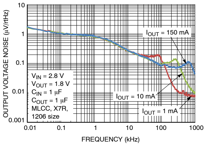
Figure 28. Output Voltage Noise Spectral Density for V_{\text{OUT}} = 1.8\text{ V} , C_{\text{OUT}} = 1\text{ }\mu\text{F}
