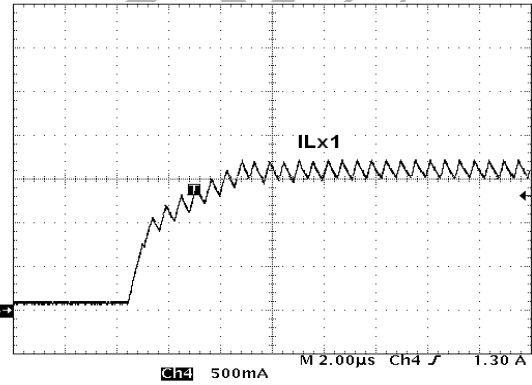
Figure 19. Current Peak Inductor Protection V_{IN} = 3.6 \text{ V} , V_{OUT1} = 1.2 \text{ V} , I_{OUT1} Short to GND, EN2 = \text{GND}
