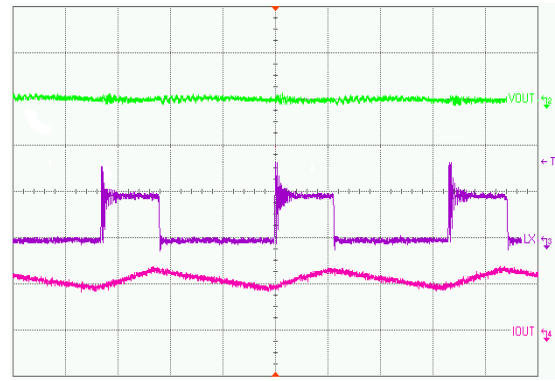
( V_{IN} = 5\text{ V} , I_{LOAD} = 500\text{ mA} , L = 3.3\text{ }\mu\text{H} , C_{OUT} = 20\text{ }\mu\text{F} ) Upper Trace: Output Ripple Voltage, 20 mV/div Middle Trace: L_X Pin Switching Waveform, 5 V/div Lower Trace: Inductor Current Waveform, 500 mA/div Time Base: 200 ns/div
