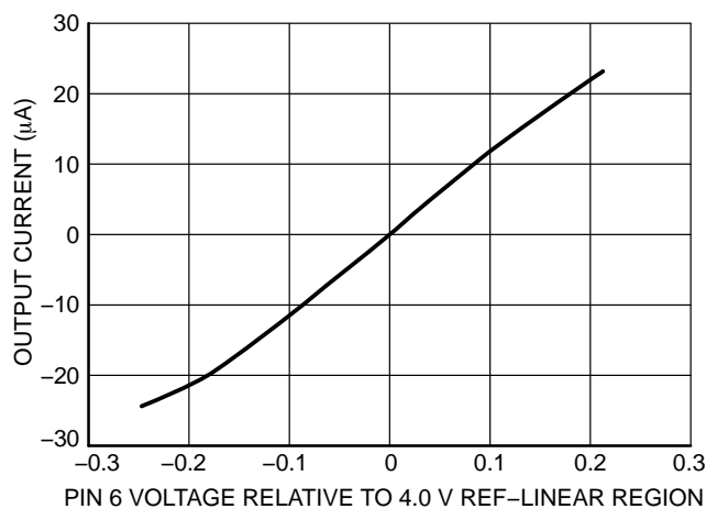
Figure 11. Voltage Amplifier Gain
