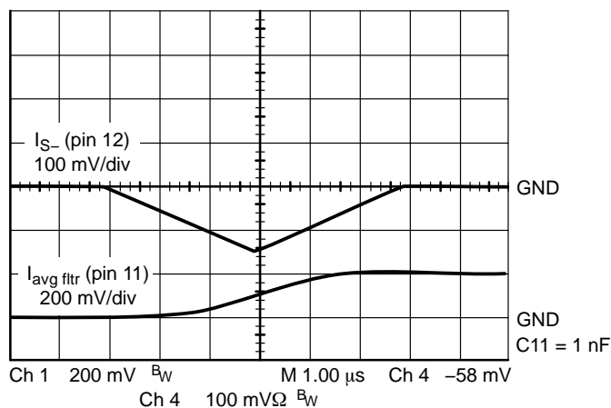
Figure 15. Current Sense Amplifier High Frequency Response
