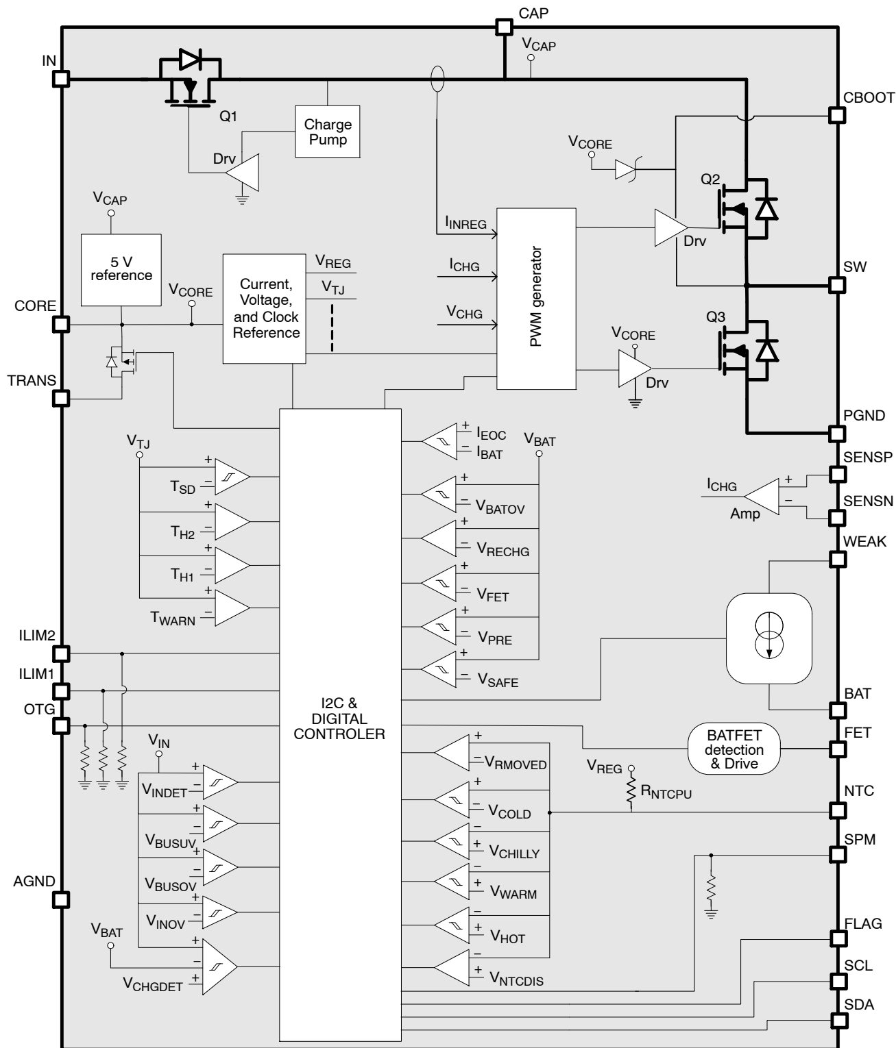
Figure 3. Block Diagram
