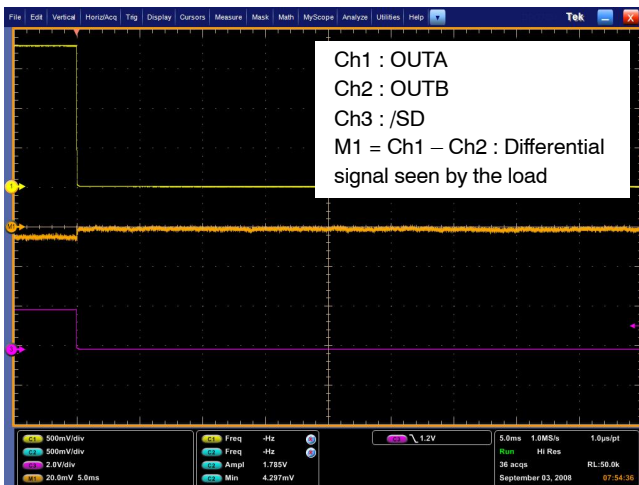
Figure 27. Zero pop noise turn off sequence with single-ended input to ground ( C_i = 100\text{ nF} , R_i = 24\text{ k}\Omega , R_f = 24\text{ k}\Omega , C_{byp} = 1\text{ }\mu\text{F} , R_L = 8\text{ }\Omega , T_{on} = \text{GND} )
