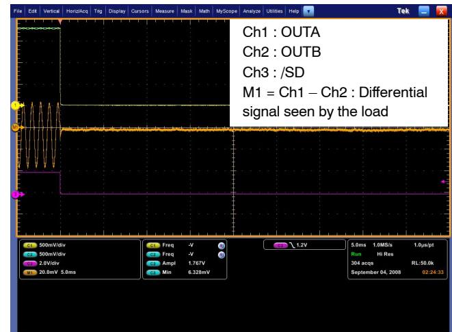
Figure 28. Zero pop noise turn off sequence with single-ended input audio source ( C_i = 100\text{ nF} , R_i = 24\text{ k}\Omega , R_f = 24\text{ k}\Omega , C_{byp} = 1\text{ }\mu\text{F} , R_L = 8\text{ }\Omega , T_{on} = \text{GND} )
