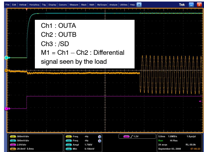
Figure 26. Zero pop noise turn on sequence with single-ended input audio source ( C_i = 100\text{ nF} , R_i = 24\text{ k}\Omega , R_f = 24\text{ k}\Omega , C_{byp} = 1\text{ }\mu\text{F} , R_L = 8\text{ }\Omega , T_{on} = \text{GND} )
