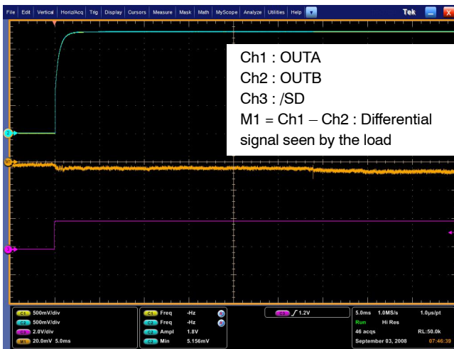
Figure 25. Zero pop noise turn on sequence with single-ended input to ground ( C_i = 100\text{ nF} , R_i = 24\text{ k}\Omega , R_f = 24\text{ k}\Omega , C_{byp} = 1\text{ }\mu\text{F} , R_L = 8\text{ }\Omega , T_{on} = \text{GND} )
