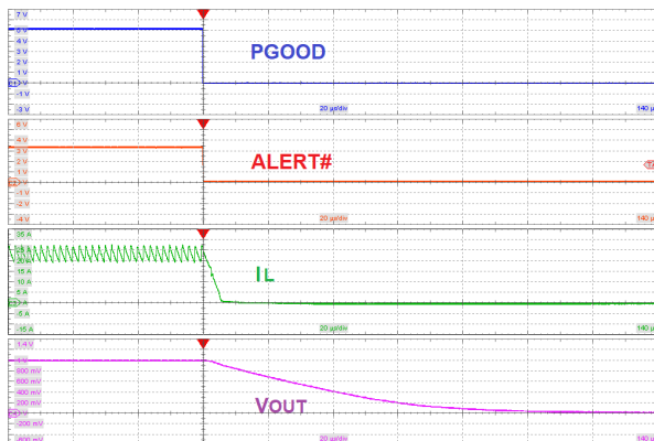
Figure 18. Over-Current Protection Response, Latch-Off, I_{VLY} = 20\text{ A}
