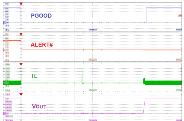
Figure 19. Over-Current Protection Response and Auto-Restart, Hiccup, I_{VLY} = 20\text{ A}
