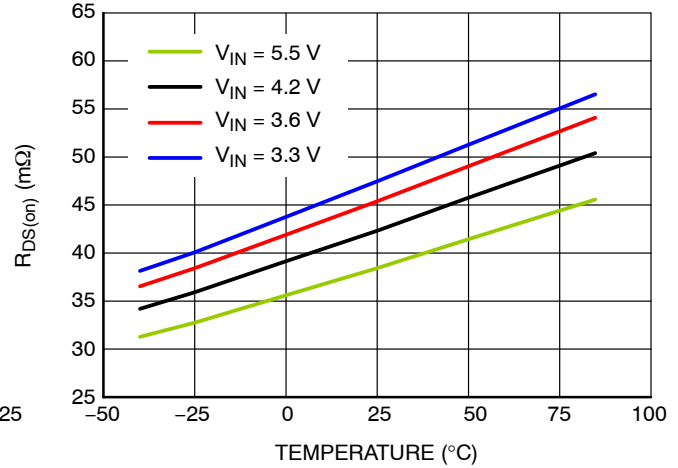
Figure 7. R_{DS(on)} ( m\Omega ) vs. Temperature ( ^{\circ}\text{C} ), I_{OUT} 2 A
