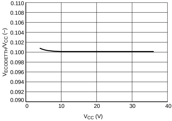
Figure 8. V_{ECOTETH}/V_{CC} Ratio at T_J = 25^\circ\text{C}
