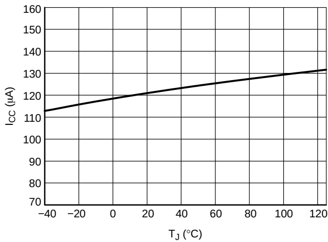
Figure 12. I_{CC} in ECO Mode, V_{CC} = 15\text{ V} , V_{ECOTETH} = 1\text{ V} , V_{SNS} = V_{REF}
