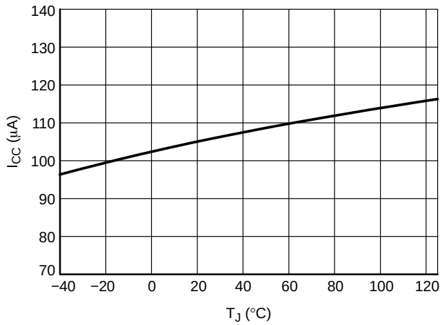
Figure 10. I_{CC} in Regulation, V_{CC} = 15\text{ V} , V_{ECOTETH} = 2\text{ V}
