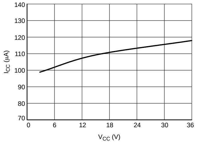
Figure 11. I_{CC} in Regulation, T_J = 25^\circ\text{C} , V_{ECOTETH} > 10\% V_{CC}
