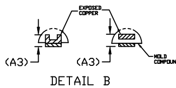
DETAIL B ALTERNATE CONSTRUCTIONS
