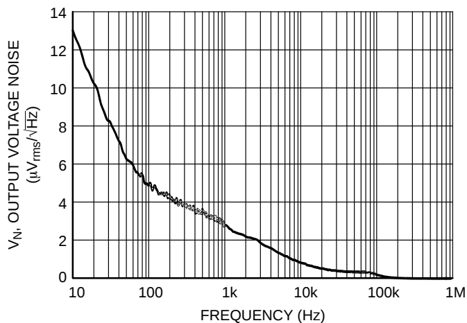
Figure 20. Output Voltage Noise, 5.5 V Version, V_{IN} = 6.5\text{ V} , I_{OUT} = 30\text{ mA} , C_{in} = C_{out} = 0.1\text{ }\mu\text{F}
