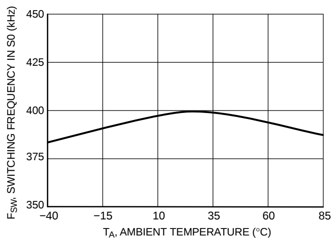
Figure 6. Switching Frequency in S0 vs. Ambient Temperature
