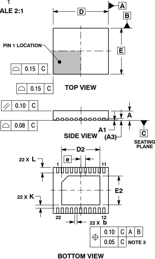
DFN22 6x5x0.9 MM, 0.5 P CASE 506AF ISSUE A
