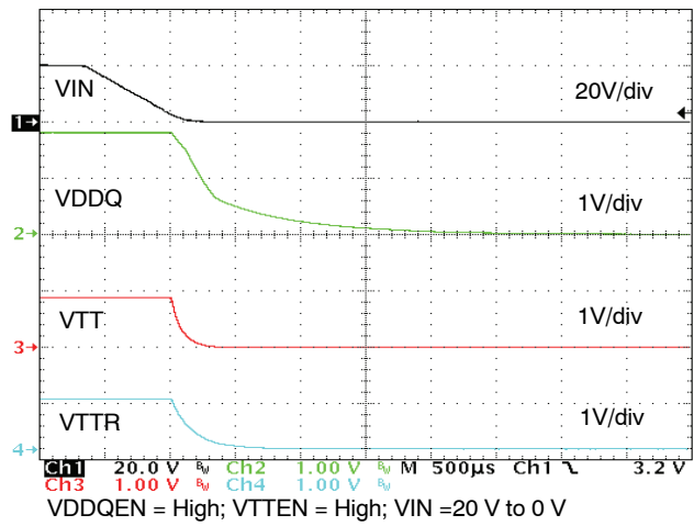
Figure 18. Powerdown Waveforms
