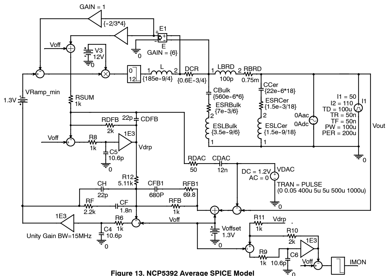
Figure 13. NCP5392 Average SPICE Model
