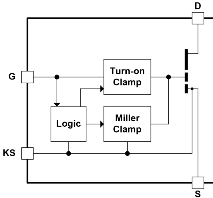
Figure 1. Block Diagram
